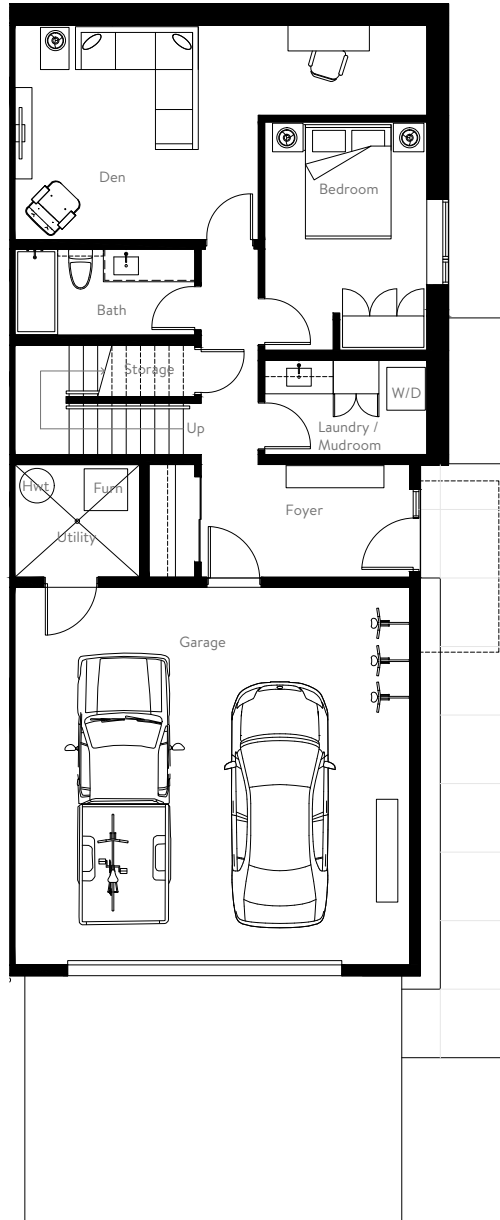
1 LEVEL 1 PLAN - UPHILL DUPLEX 1/4" = 1'-0"
